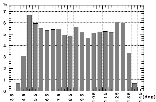
Figure 3. The best determinations of \gamma in each technique.
