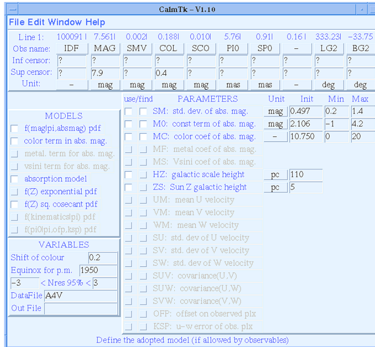
Figure 1. The user interface to the calibration program.
