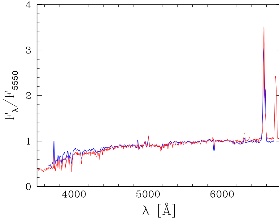
Figure 5.20: The comparison between the average spectrum of e(a) galaxies in the sample of Poggianti & Wu (2000) (thick line) and a simulated spectrum (thin line).
