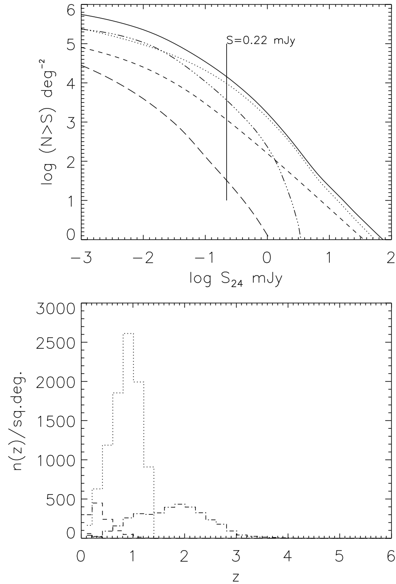
Figure 7.4: 24\mu\text{m} source counts and redshift distributions, at 0.22 mJy, the expected 5\sigma confusion limit. The dotted line refers to starbursts, the dashed one is for spirals, the dot-dashed one for star-forming spheroidal galaxies, long dashed line for passively evolving spheroidal galaxies.
