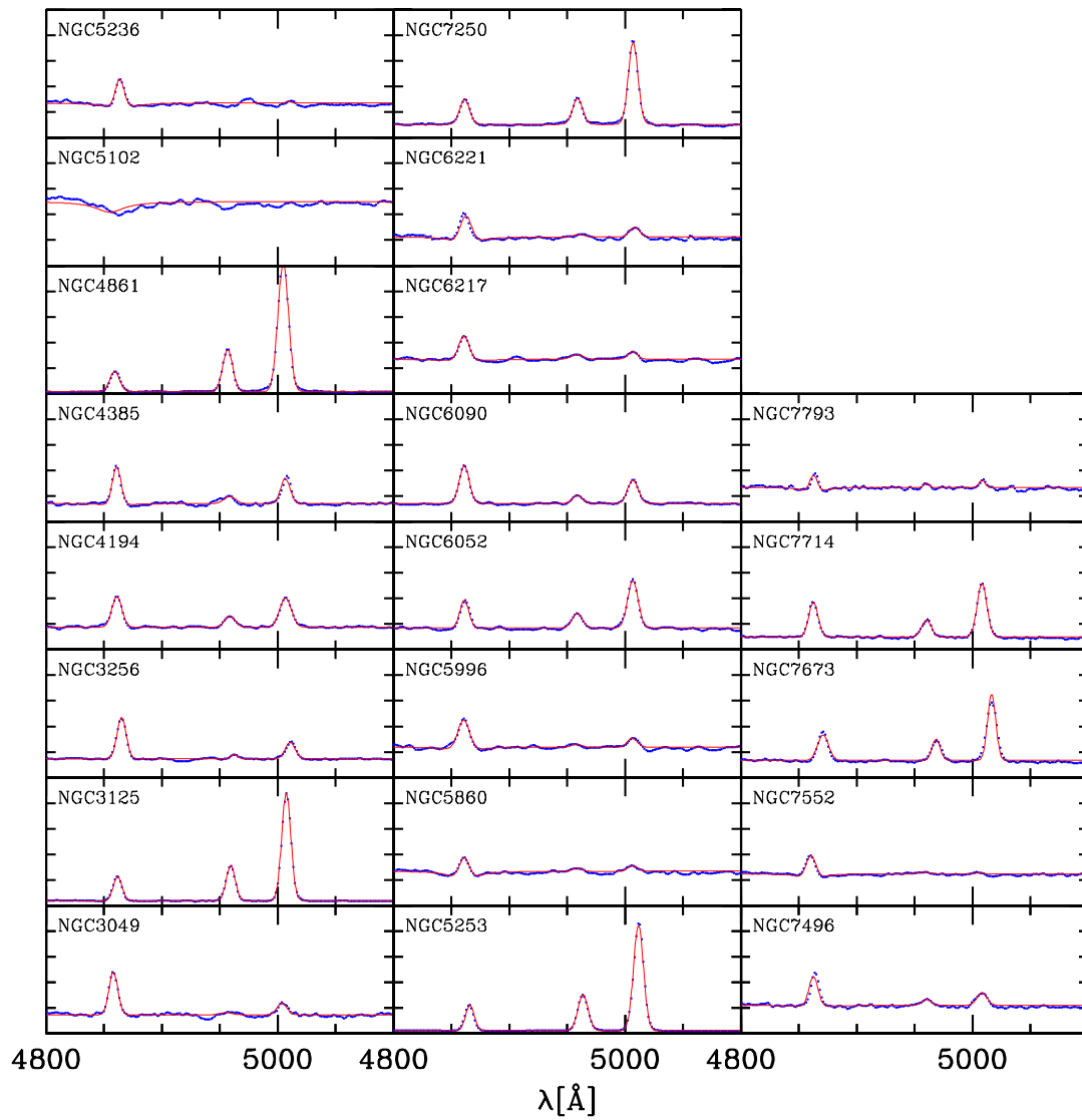
Figure A.6: As fig. A.5, but for the remaining objects.
