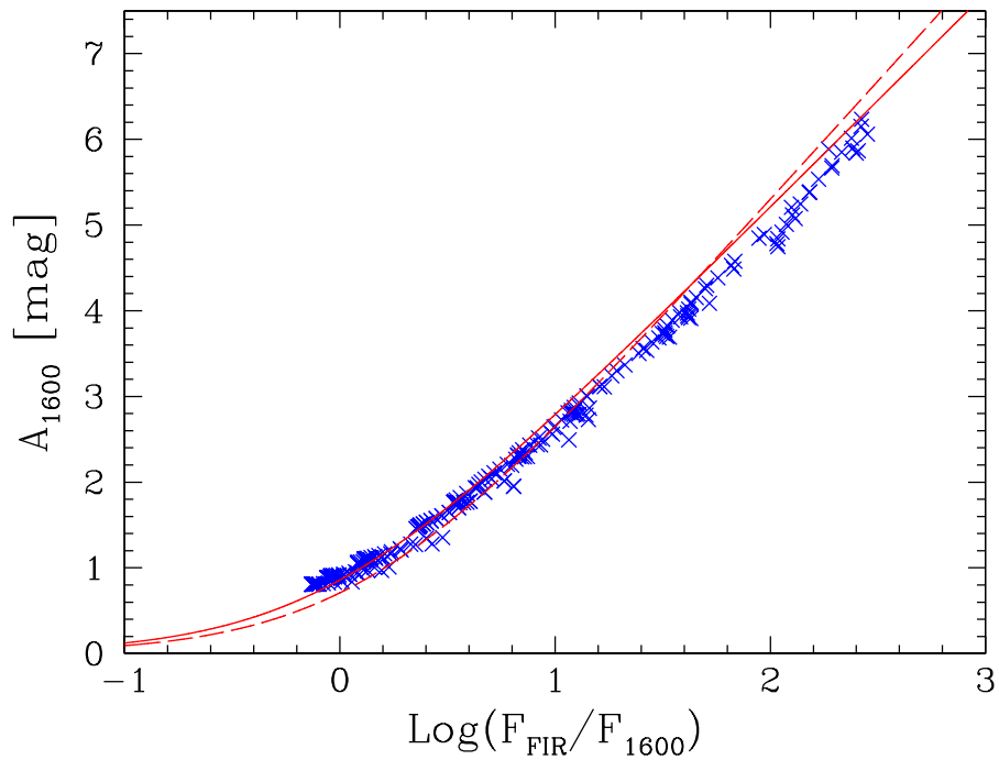
Figure 5.14: The comparison between real A_{1600} derived from the models and the ratio F_{\text{FIR}}/F_{1600} in simulated starburst (crosses). The solid line shows the relation derived by MHC99 (eq. 4.7), while the dashed line is the relation that we derived for normal galaxies (eq. 4.10) assuming A_{1600} = A_{2000}/0.9 .
