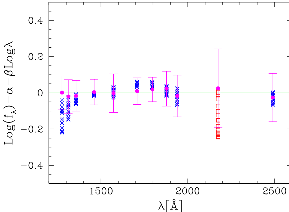
Figure 5.12: The residuals d_\lambda = \log f_\lambda - \alpha - \beta \log \lambda from the fitting of UV spectra for models with \beta > -1.5 and \text{EW}(\text{H}\alpha + [\text{N II}]) < -40 \text{ \AA} versus the wavelength in the 10 spectral bands (crosses) and around 2175 \text{ \AA} (empty squares). Filled circles with error-bars show the deviations for W02 galaxies.
