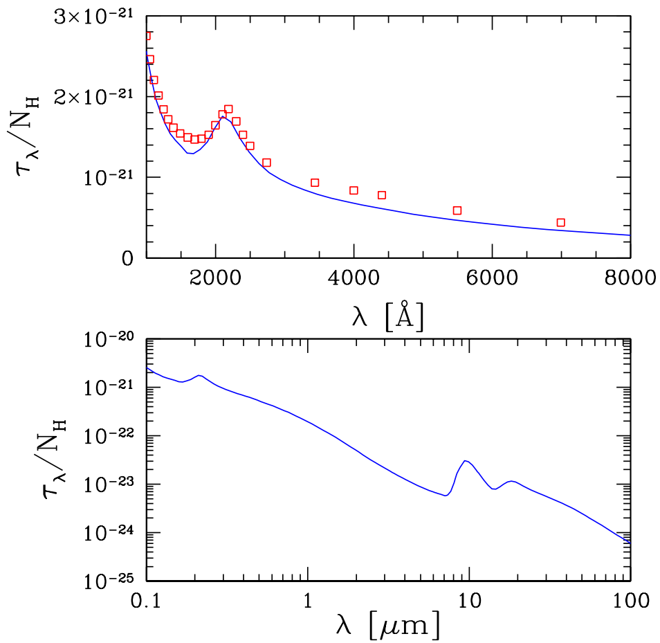
Figure 3.3: Extinction law (solid line) for the dust mixture that we adopted in this work. The mixture adopted give rise to an extinction law very similar to the galactic one (open squares) (Pei, 1992).
