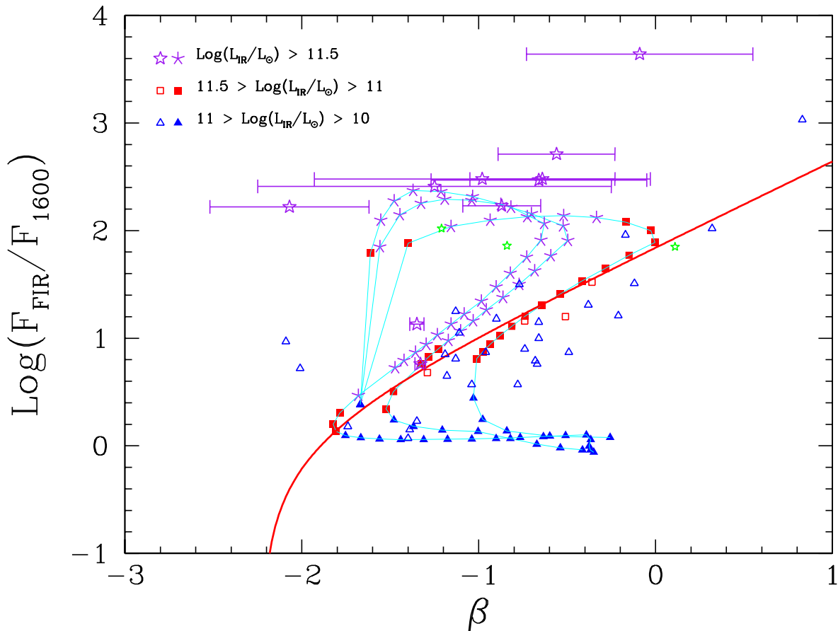
Figure 5.16: The F_{\text{FIR}}/F_{\text{UV}} vs the UV spectral index for simulated VLIRGs. Galaxies from Wu et al. sample with L_{\text{IR}} > 10^{10} L_{\odot} are plotted with small symbols (open squares, open triangles, and open stars), while VLIRGs from Goldader et al. (2002) are shown with large open stars. Error bars indicate the uncertainties in the \beta determination. The evolution of models for three different burst timescales are compared with observations at different times from the burst set-up. The reddest sequence corresponds to t_b = 50 Myr, the bluest one corresponds to t_b = 10 Myr; in the middle there are the models with t_b = 20 My.
