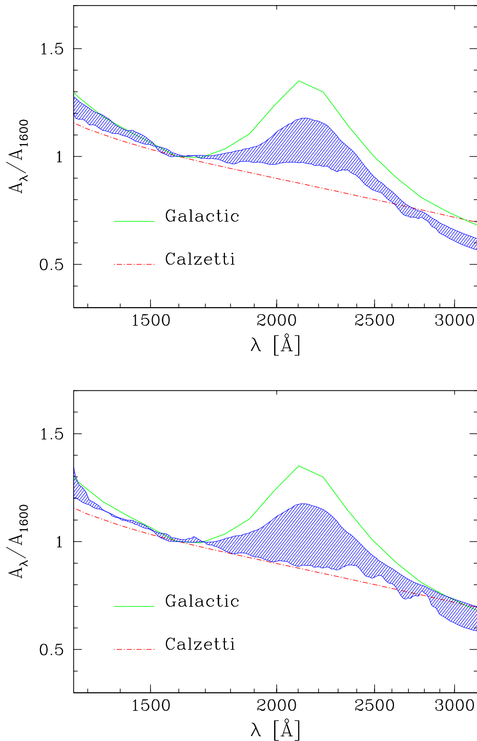
Figure 5.11: The attenuation curve of simulated UV-bright starbursts. The thick continuous line shows the galactic extinction law, while the dot-dashed line refers to the Calzetti attenuation law. The shadowed regions show the variation of the attenuation A_\lambda of the models. Upper panel: model A, lower panel: model B.
