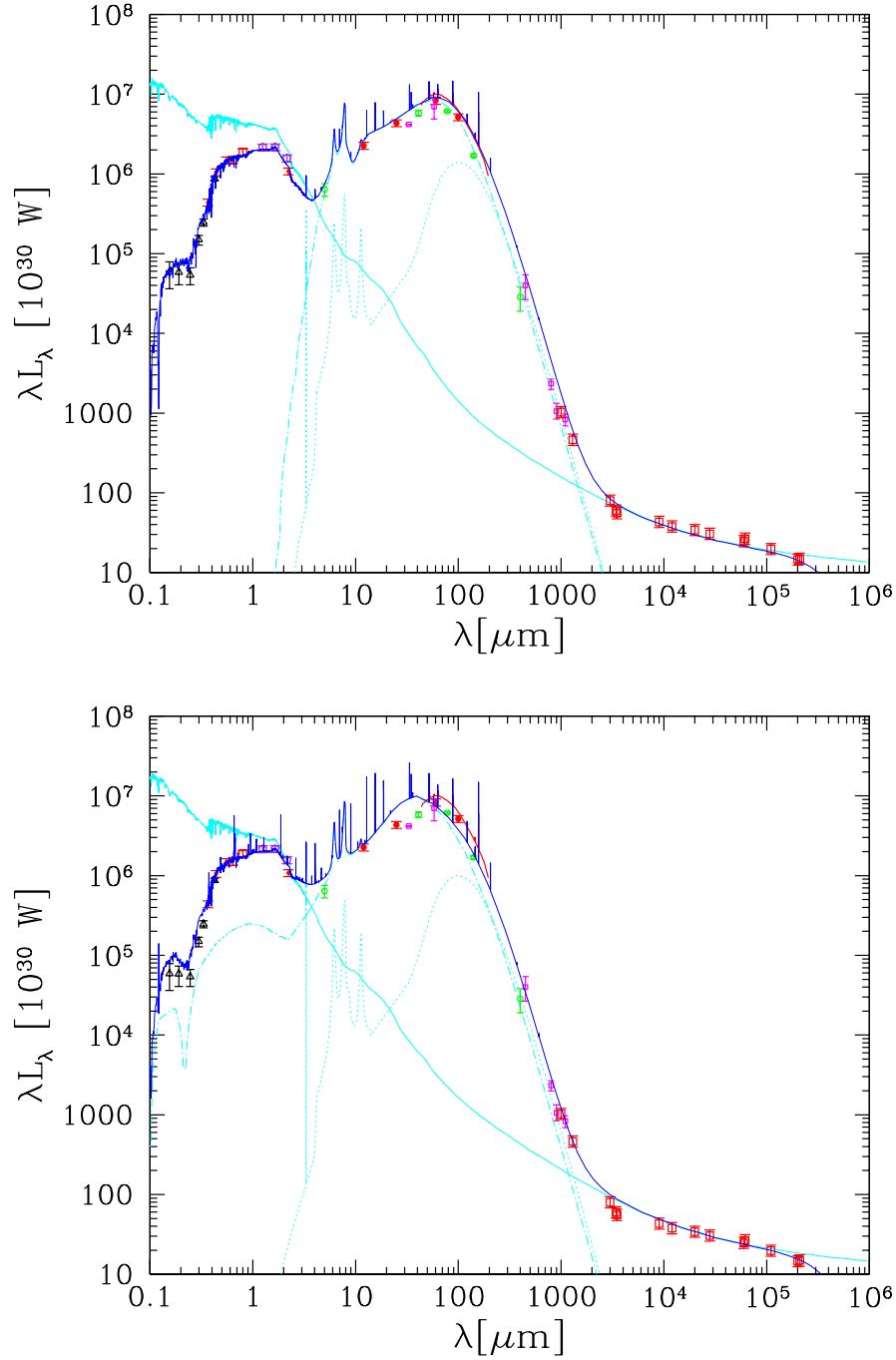
Figure 3.6: The global spectral energy distribution of M82, for the model A (upper panel) and model B (lower panel). Photometric data are from: UV: Code & Welch (1982) (open triangles); NIR: 2MASS (Jarrett et al., 2003); FIR spectrum: Colbert et al. (1999); IRAS: Soifer et al. (1989); Sub-mm and other IR data: Telesco & Harper (1980), Jaffe et al. (1984), Hughes et al. (1990), Radio: Huang et al. (1994). The different lines represent: the unextinguished continuum (thin solid), the emission of cirrus (dotted), the radiation emerging from molecular clouds (dot-dashed), and the final SED (thick solid).
