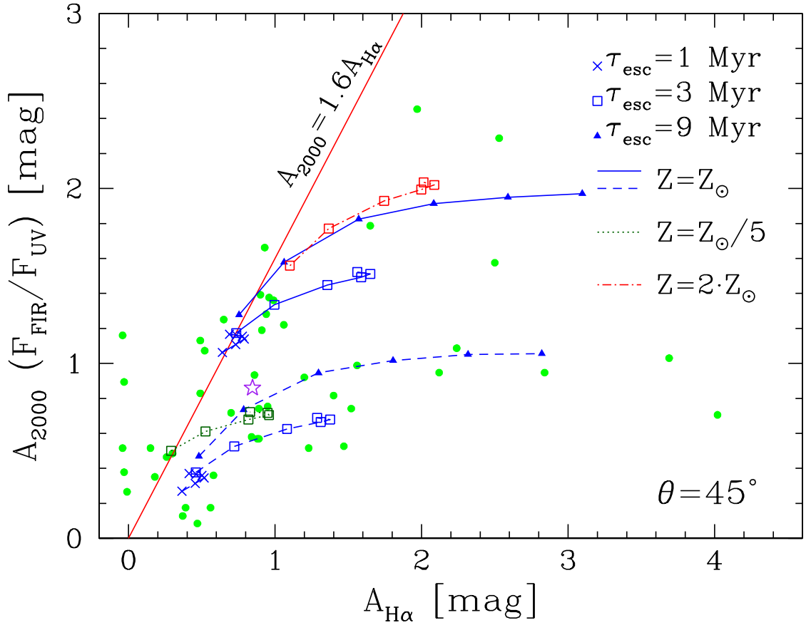
Figure 4.5: On the ordinate, A_{2000} derived from the ratio F_{\text{FIR}}/F_{2000} (using eq. 4.8); on the abscissa, A_{\text{H}\alpha} from Balmer decrement. Filled circles show SFG sample data. Lines connect models with the same M_{\text{G}} and star formation history, but different \tau_{\text{MC}} . Solid lines: M_{\text{G}} = 10^{11} M_{\odot} , \nu_{\text{sch}} = 0.3 \text{ Gyr}^{-1} , \tau_{\text{inf}} = 18 \text{ Gyr} , solar metallicity; dashed lines: M_{\text{G}} = 10^{10} M_{\odot} , \nu_{\text{sch}} = 0.7 \text{ Gyr}^{-1} , \tau_{\text{inf}} = 6 \text{ Gyr} , solar metallicity. To emphasize the dependence on metallicity, we show the first model (solid lines) for \tau_{\text{esc}} = 3 \text{ Myr} but Z = 0.04 (dot-dashed line) or Z = 0.004 (dotted line). For simplicity only models with \theta = 45^{\circ} are shown here.
