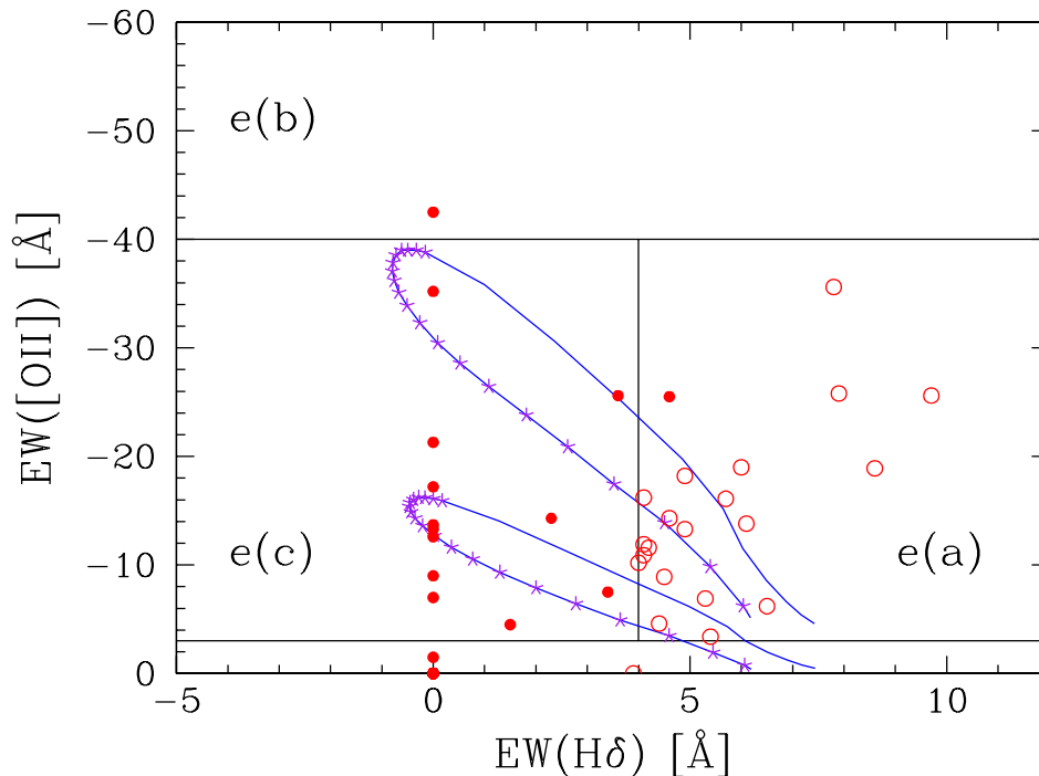
Figure 5.19: The evolution of IR starburst models on classification diagram of the [O II]3727 equivalent width versus H \delta equivalent width, compared to the observed VLIRGs by Poggianti & Wu (2000) (filled and open circles). The models shown here have t_b = 20 Myr; models with a lower [O II]3727 emission have a solar metallicity, the other have Z = 0.4Z_\odot . Observed object with H \delta unobserved or nearly filled are placed at \text{EW}(\text{H}\delta)=0 .
