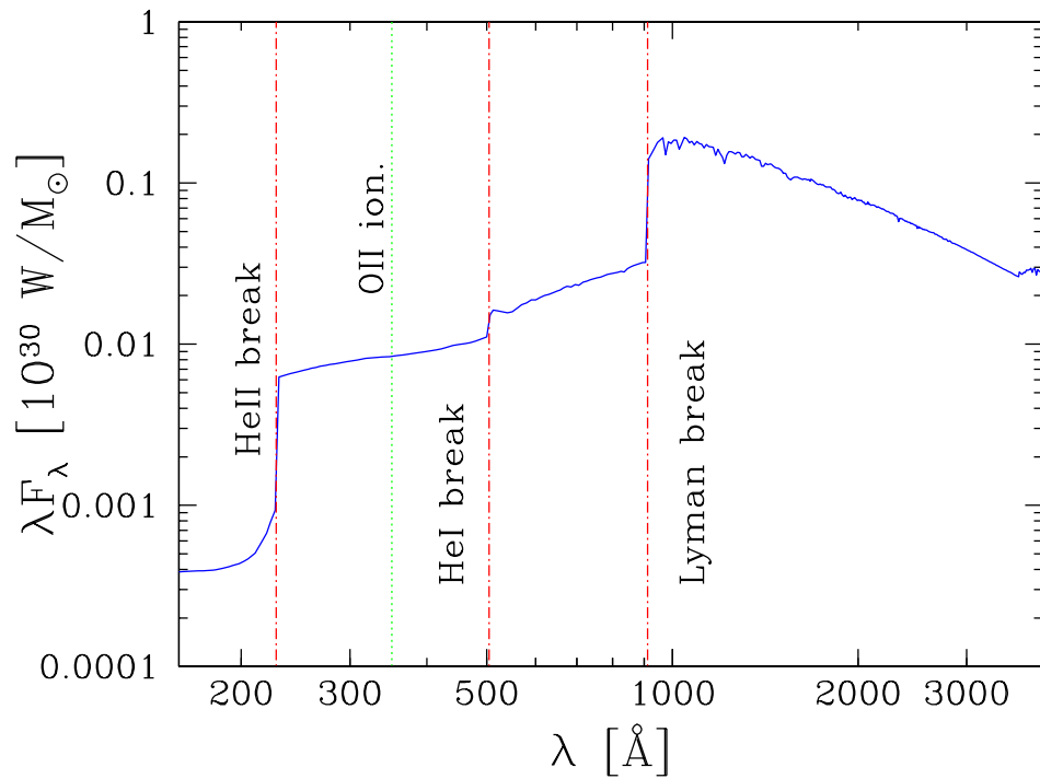
Figure 2.2: The SED of a typical young SSP (5 Myr old and Z=0.008 ). The dot-dashed vertical lines show the position of spectral discontinuities corresponding to the H, He I and He II ionizing energies (namely Lyman break, He I and He II break). The dotted line shows the position of O II ionizing energy.
