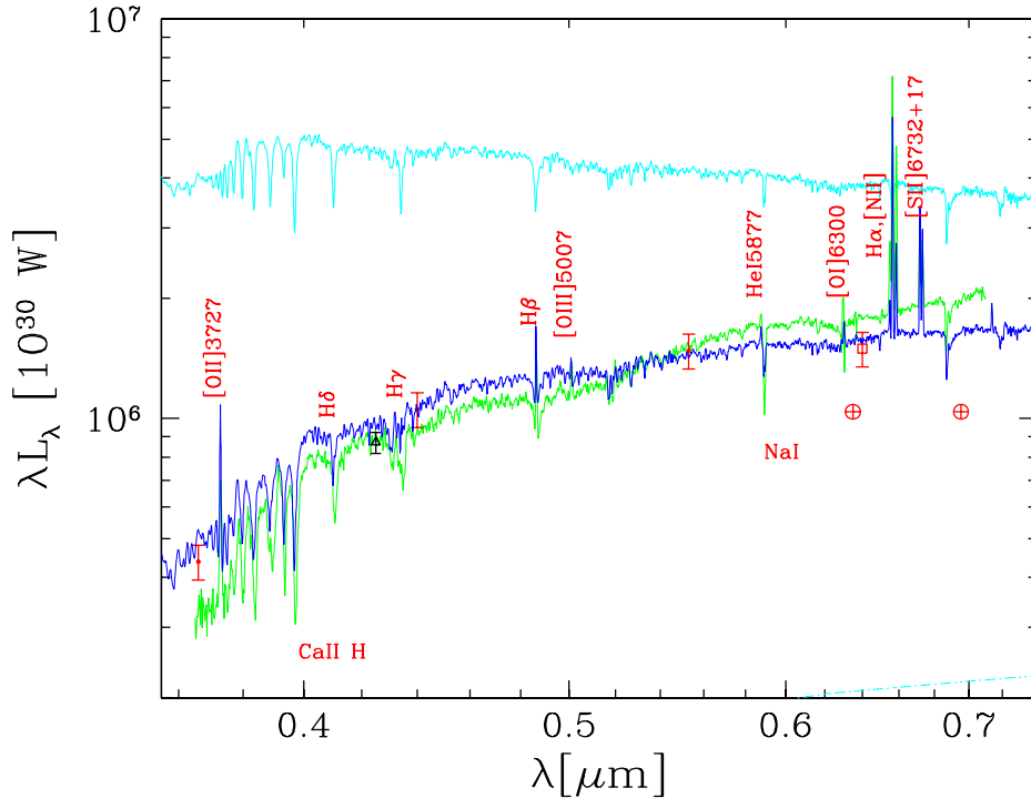
Figure 3.7: Optical SED of M82. The simulated SED (thick line) is compared to a spectrum from Kennicutt (1992), the latter normalized to have a flux 2.19 \cdot 10^{32} \text{ W}/\text{\AA} at 5500 \text{ \AA} . Some emission lines are highlighted, as well as the stellar absorption doublet Ca II H, the interstellar absorption of Na I and two telluric features. The resolution power \lambda/\Delta\lambda used (1000) is very similar to the one in the observed spectrum.
