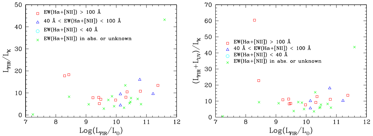
Figure 5.5: Left panel: the ratio FIR/K' vs the FIR luminosity for the W02 sample. Right panel: the ratio (FIR+UV)/K' vs the FIR luminosity.
