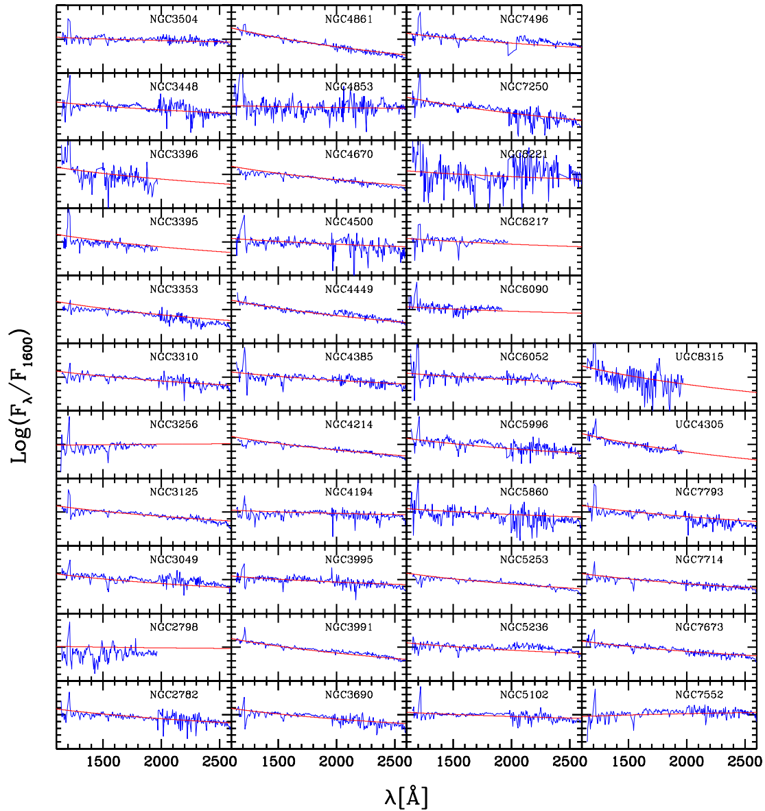
Figure A.2: As fig. A.1, but for the remaining objects.
