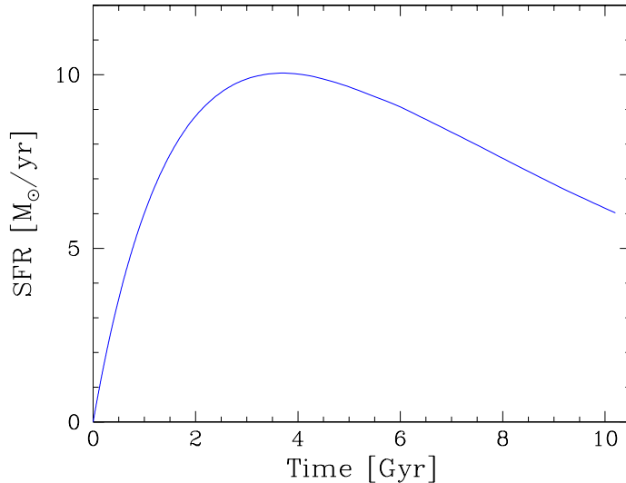
Figure 3.8: The star formation history of M99.
