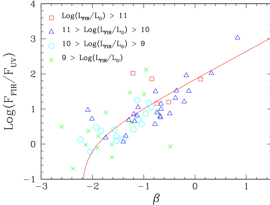
Figure 5.3: The ratio F_{\text{FIR}}/F_{2000} vs. \beta for the UV selected sample. Different symbols refer to different FIR luminosity.
