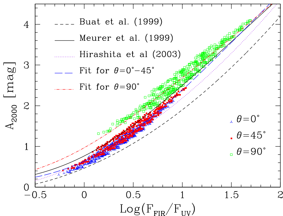
Figure 4.7: UV attenuation vs the ratio F_{\text{FIR}}/F_{\text{UV}} ; lines refer to our fits and relations proposed in other works.
