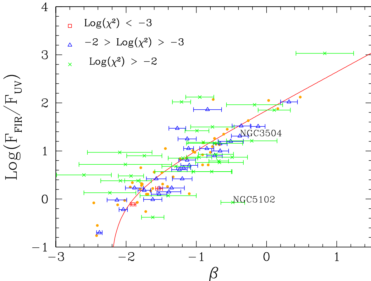
Figure 5.2: The ratio F_{\text{FIR}}/F_{2000} vs. \beta for the W02 sample. Different symbols (open squares, open triangles and crosses) refer to different quality of the power-law fitting of UV spectra; error bars show the statistical error on the \beta determination. Small filled circles are data published in MHC99, while the thick line shows the mean relationship provided by MHC99.
