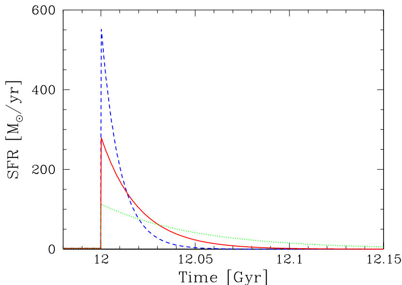
Figure 5.15: The star formation rate during the burst of simulated IR luminous galaxies. Different lines refer to different e-folding times: dashed for t_b = 10 Myr, continue line for t_b = 20 Myr and dotted for t_b = 50 Myr.
