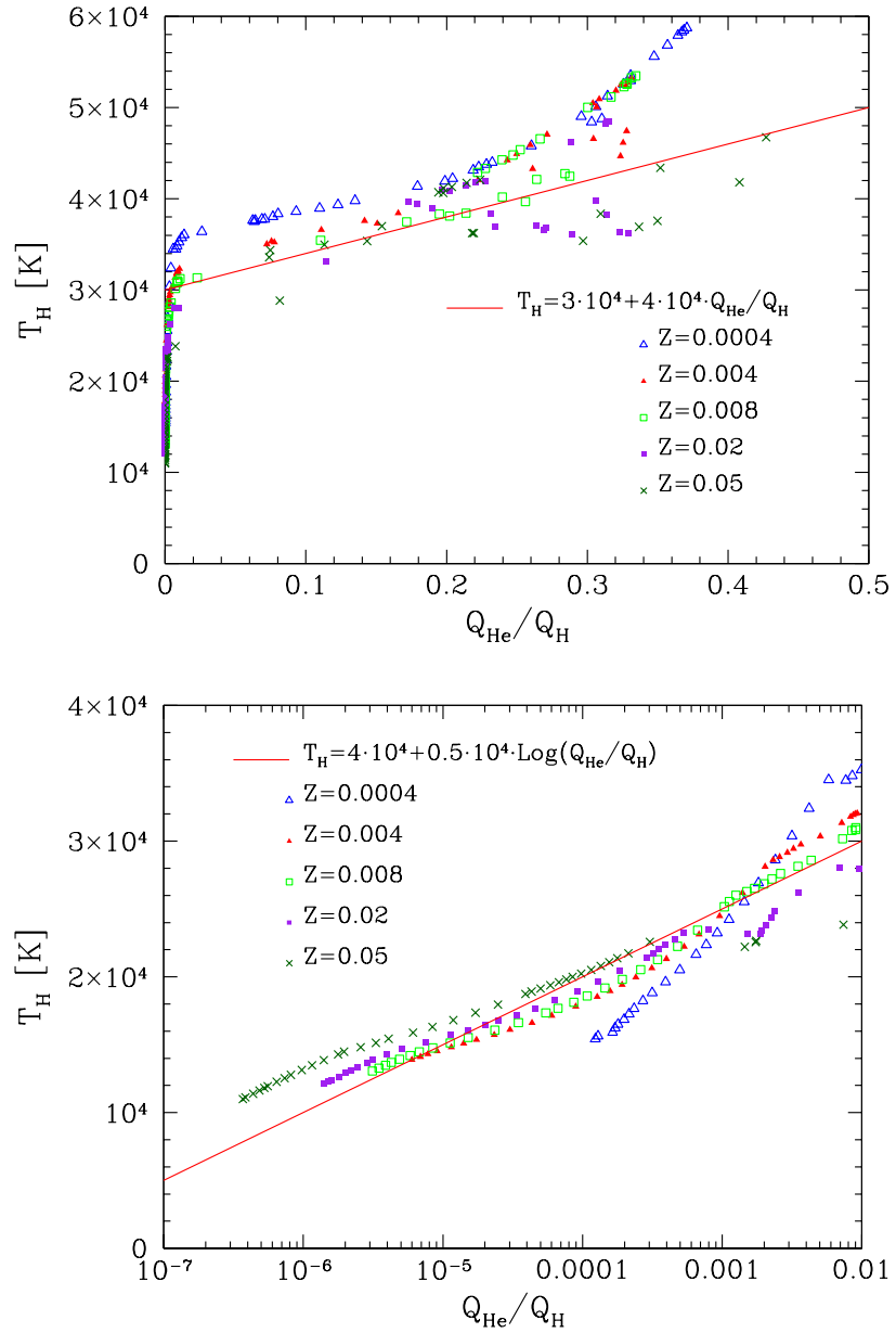
Figure 2.3: Temperature of ionizing continuum T_H as a function of Q_{\text{He}}/Q_{\text{H}} for young SSPs of different ages (from 0.1 to 30 Myr) and metallicity (points). The lines refer to the analytical fit (eq. 2.5).
