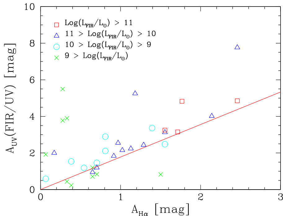
Figure 5.7: The comparison between the attenuation at 1600 \text{ \AA} derived from equation 4.7 versus the attenuation in H\alpha derived from the Balmer decrement in the sample of W02. Galaxies are represented with different symbols according to their FIR luminosity.
