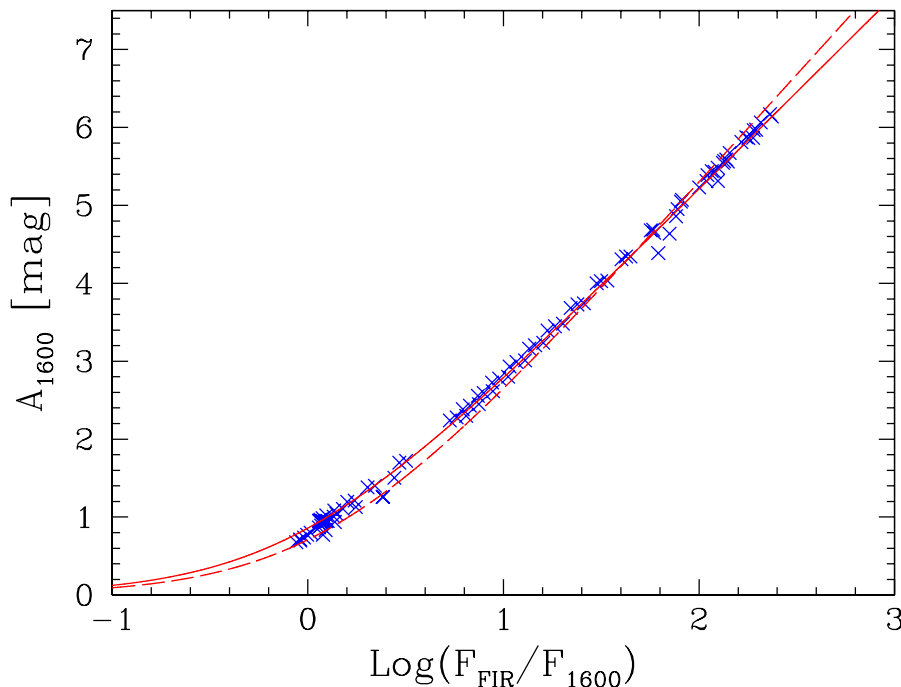
Figure 5.18: The comparison between real A_{1600} derived from the models and the ratio F_{\text{FIR}}/F_{1600} in simulated IR starburst (crosses) as in figure 5.14. The solid line shows the relation derived by MHC99 (eq. 4.7), while the dashed line is the relation that we derived for normal galaxies (eq. 4.10) assuming A_{1600} = A_{2000}/0.9 .
