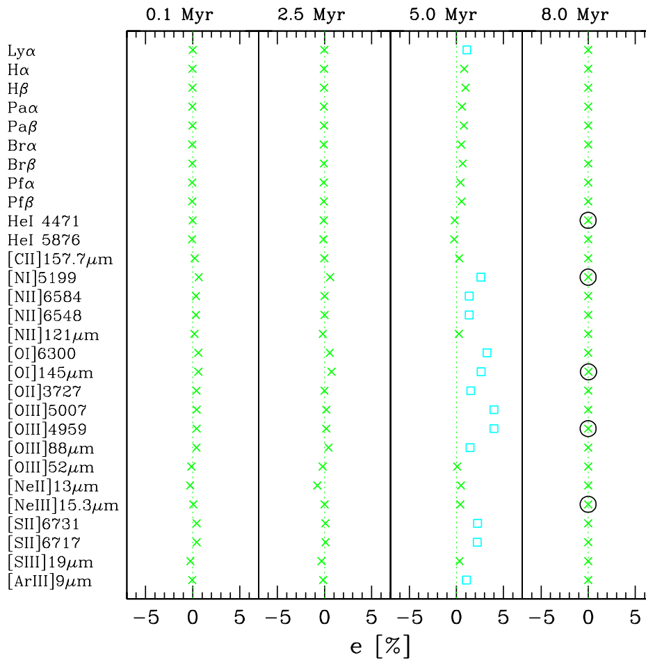
Figure 2.6: Differences between H II region models excited by SSP spectra with and without high energy photons. Crosses are for difference smaller than 1%, empty squares for difference between 1% and 5%; circled symbols refer to very low luminosity lines. Gas and star metallicity is 0.008.
