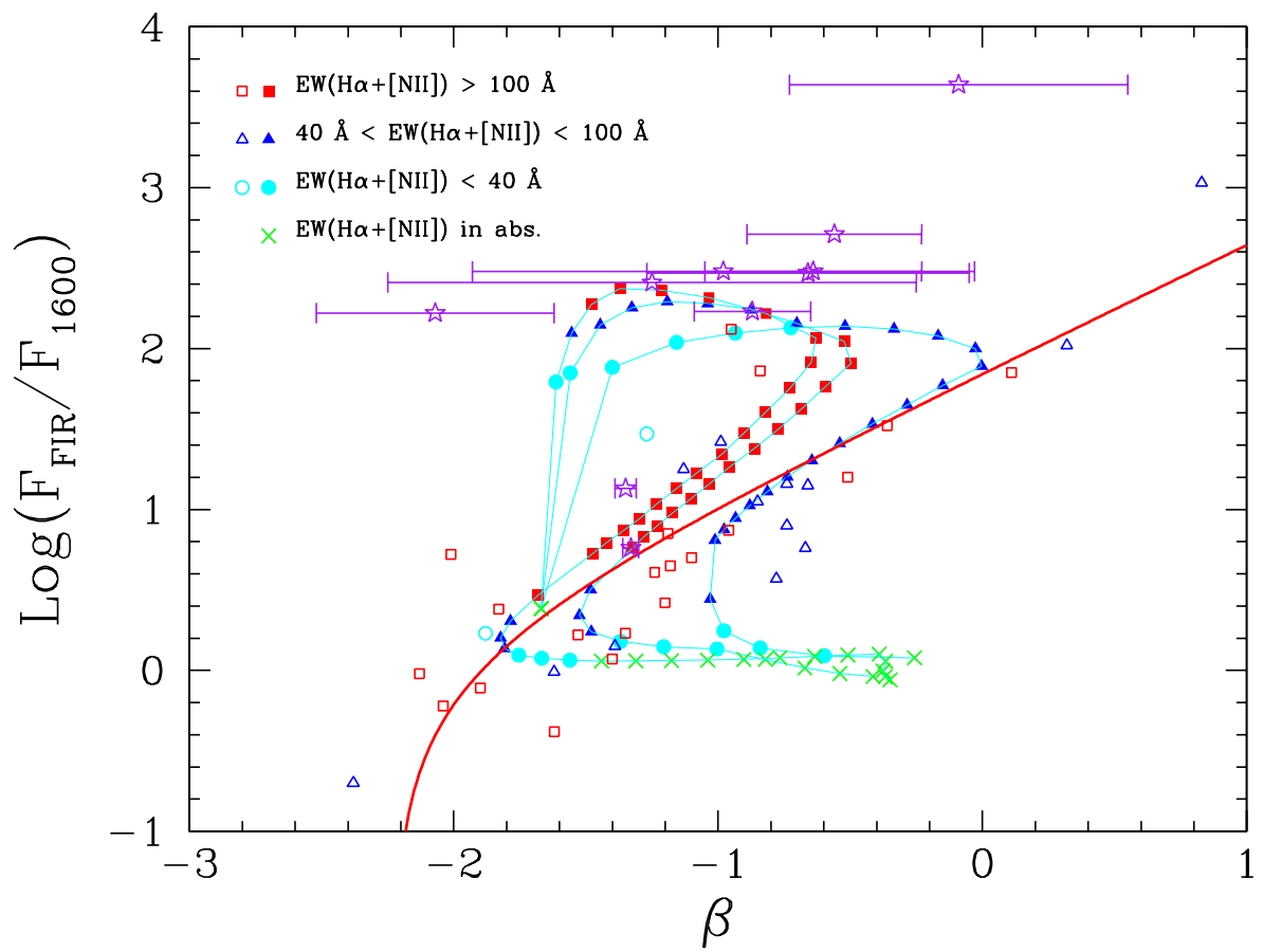
Figure 5.17: As figure 5.16, but putting in evidence the value for the equivalent width of \text{H}\alpha + [\text{NII}] .
