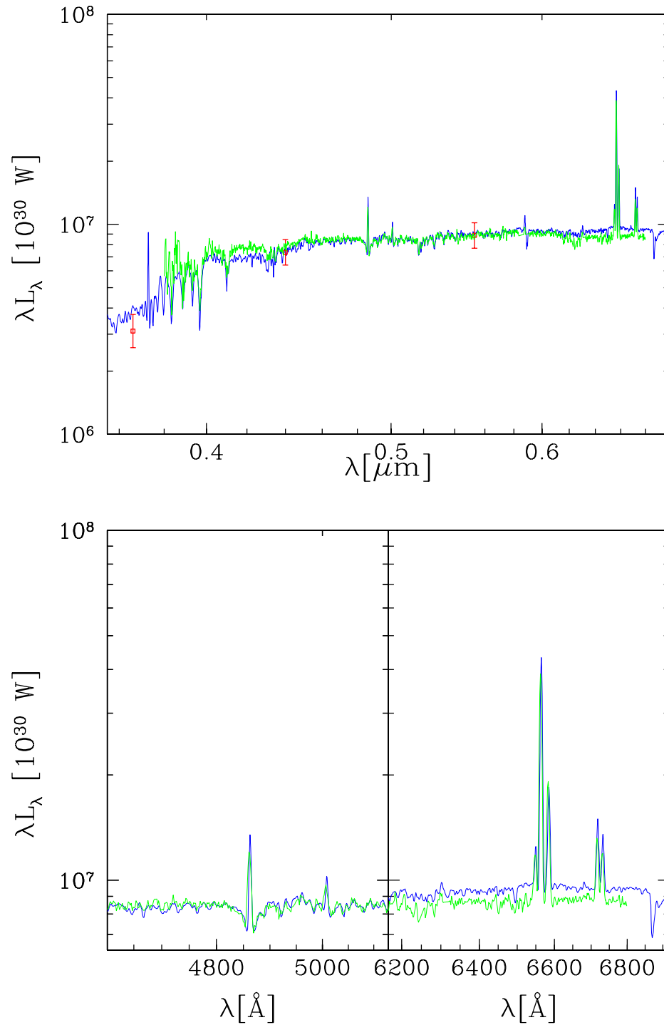
Figure 3.10: The optical spectral energy distribution of M99. Upper panel: the SED of the model (thick solid) compared with the observed spectrum (thin line). Bottom panel: detailed view of the spectrum around H \beta (left) and H \alpha (right).
