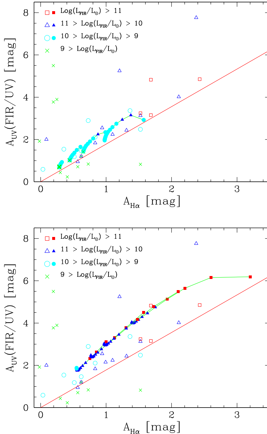
Figure 5.13: The comparison between A_{1600} derived from the FIR/UV ratio versus the attenuation in H \alpha derived from the Balmer decrement. Galaxies of W02 sample are represented with different symbols according to their FIR luminosity; connected symbols show the time evolution of models of the case A (upper panel) and the case B (lower panel).
