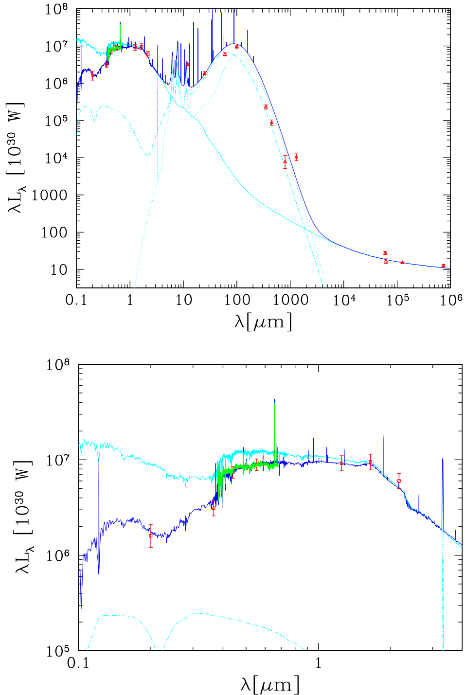
Figure 3.9: The spectral energy distribution of M99 (upper panel: the global SED; bottom panel: the SED from UV to NIR). The different lines represent: the unextincted continuum (thin solid), the emission of cirrus (dotted), the radiation emerging from molecular clouds (dot-dashed), and the final SED (thick solid).
