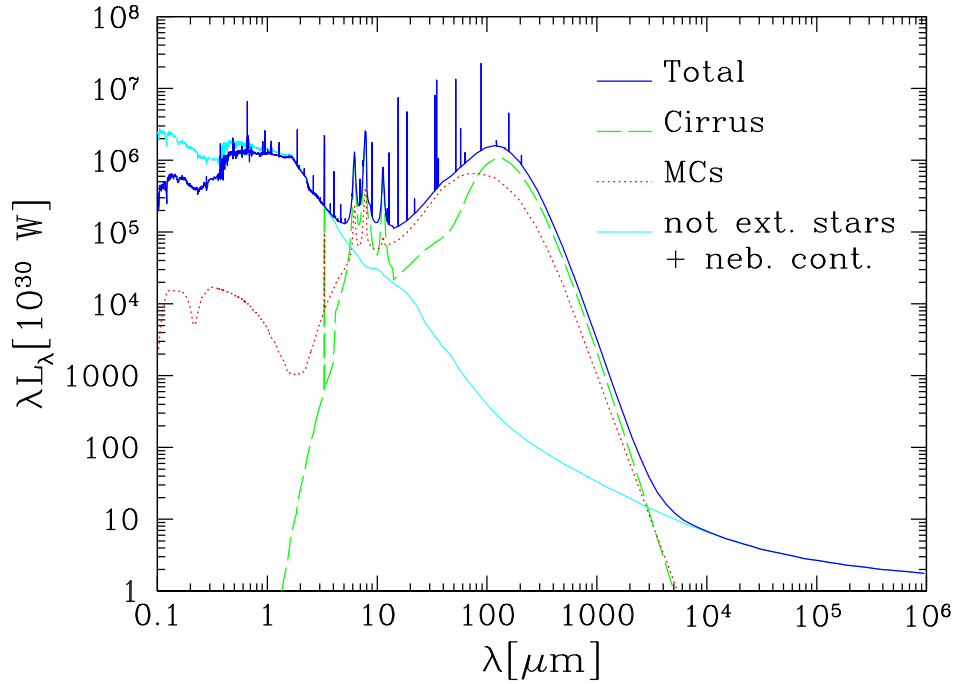
Figure 4.3: The global spectral energy distribution of the reference model (see table 4.1) with inclination \theta = 45^\circ . Different lines show different contributions.
