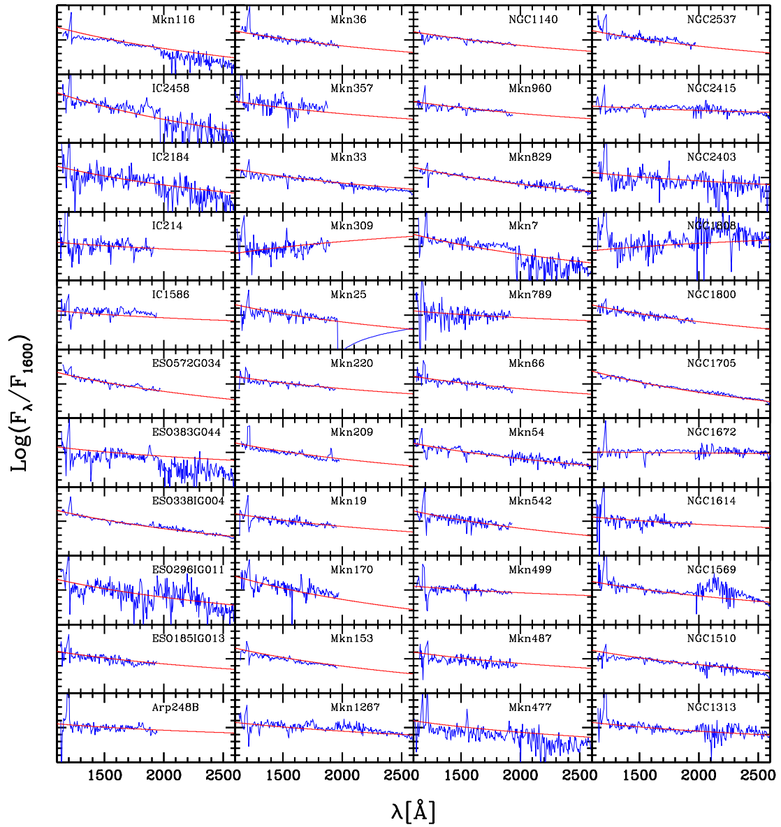
Figure A.1: UV spectra of first 44 objects of the sample compared with the appropriate fit.
